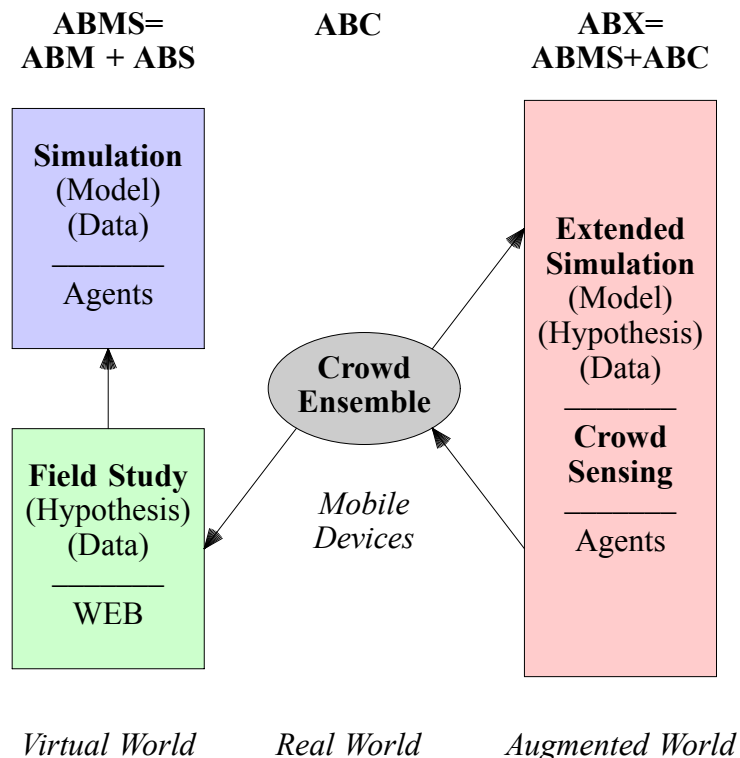
Figure 1: (Left) Traditional ABMS with separate field studies (Right) New ABX combining modelling, simulation, and field studies via crowd sensing
