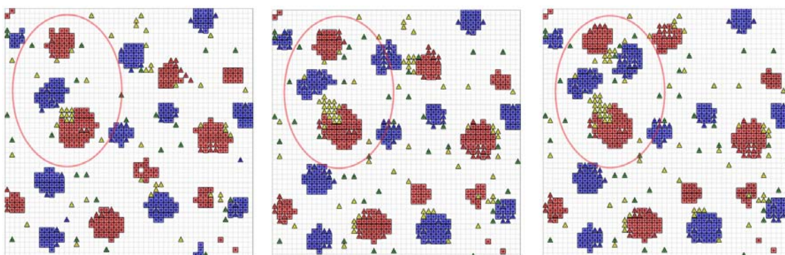
Figure 4: Simulation world at different simulation times (500/1000/1500 steps) consisting of 200/200 a/b class agents (blue/red squares) all with S=(1,-1,-1,1) and r=3 parameter settings and additionally up to 200 digital twins (triangles with colour based on individual S/r parameters)
