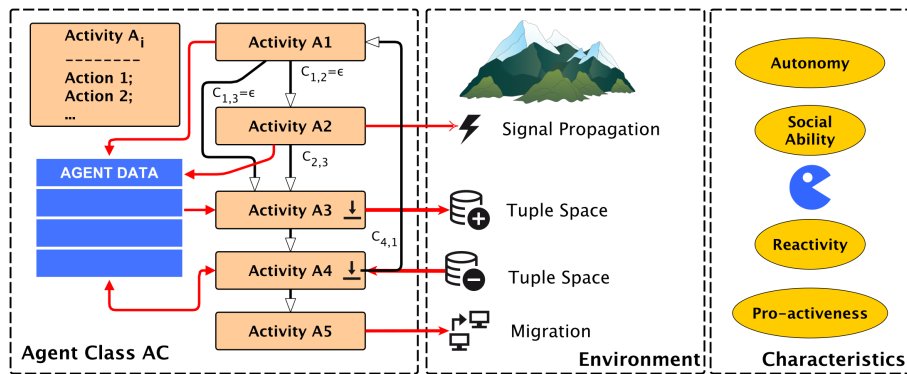
Figure 1. (Left) Agent Behaviour Model: Activity-Transition Graph and body variables (agent data) compose an agent class. (Right) Interaction with the environment (agents and platform) via tuple space access, signals, and mobility.
